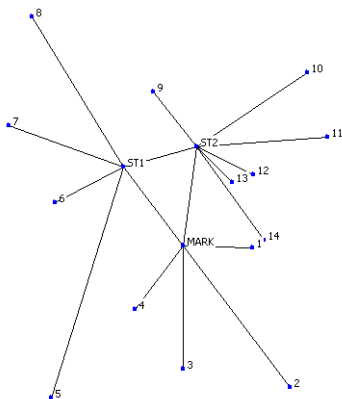
Figure 2-1. Surveying Scheme Used
